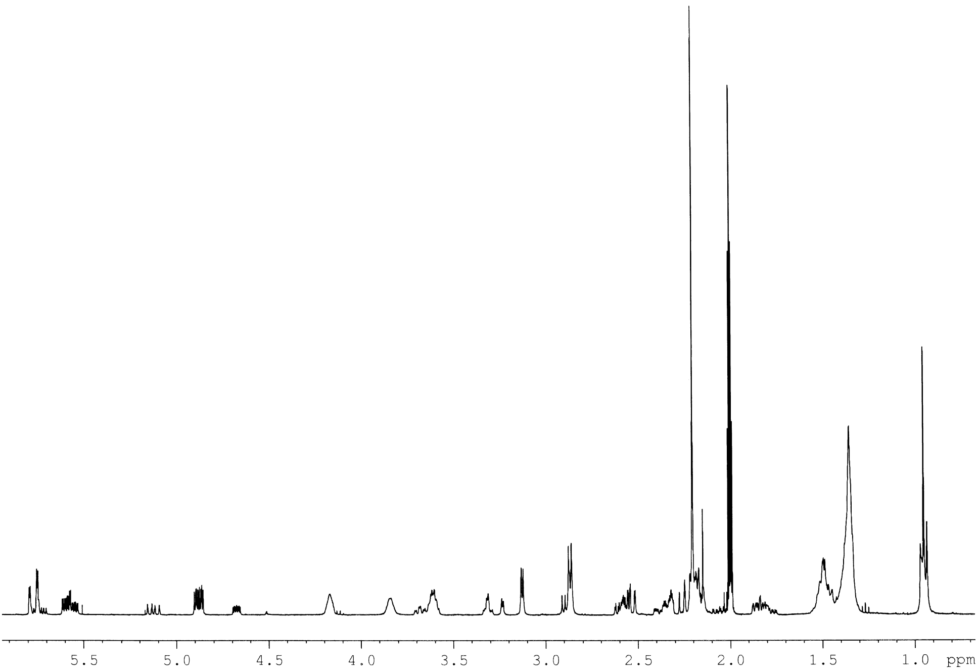
1H NMR spectrum (400 MHz, CD3CN) of synthetic 1
