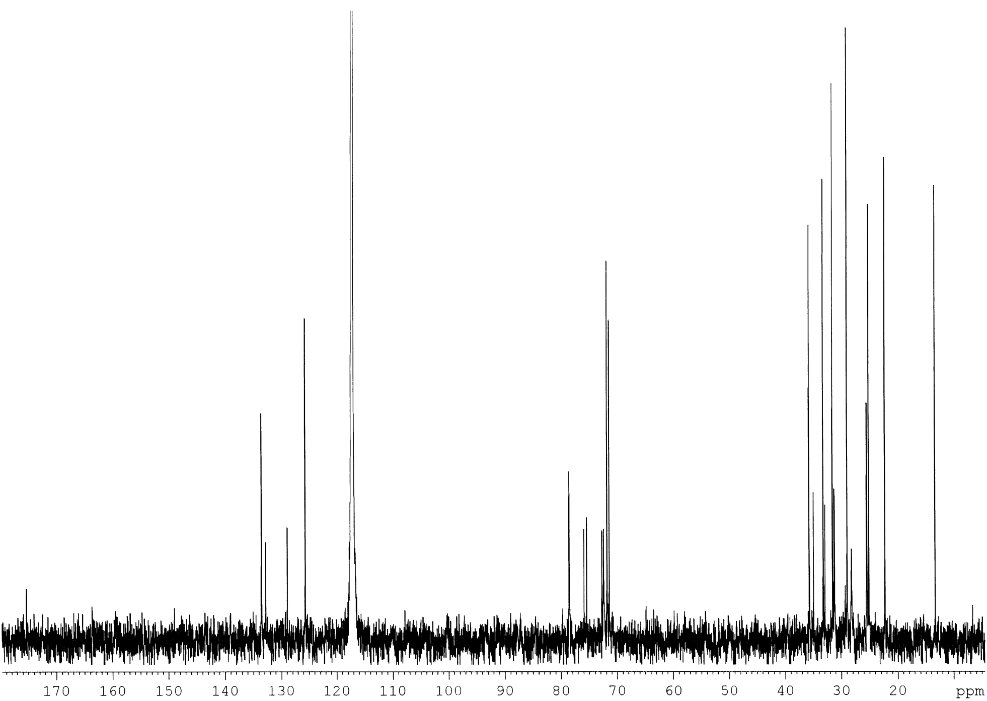
13 C NMR spectrum (100 MHz, CD 3 CN) of synthetic 1
